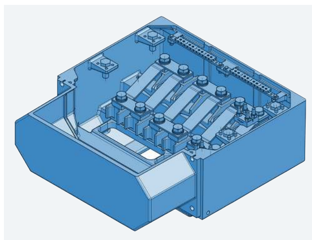
Terminal box 1XB1 631
