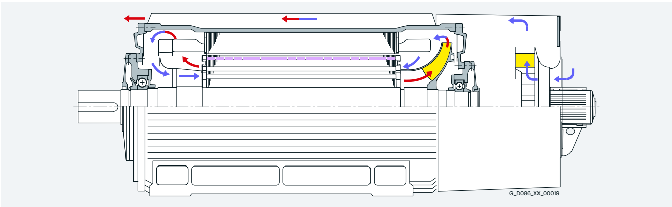
Basic structure of the air-cooled HT-direct motor 1FW4
