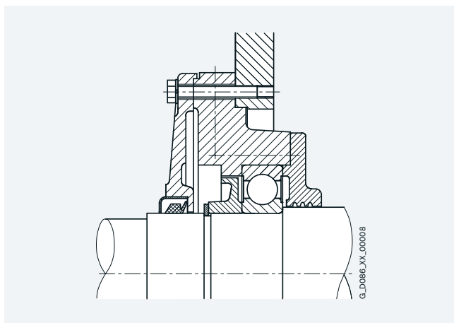
Bearing at DE (fixed bearing)
