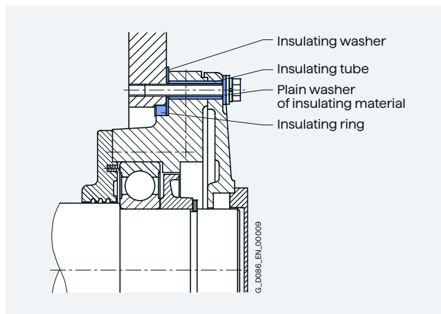
Bearing at NDE (floating bearing): Electrically insulated bearing cartridge, backlash-free adjusted deep-groove ball bearing
