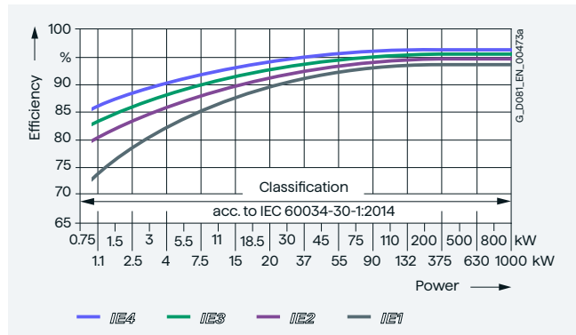
IE1-IE4 efficiencies, 4-pole, 50 Hz, according to power
