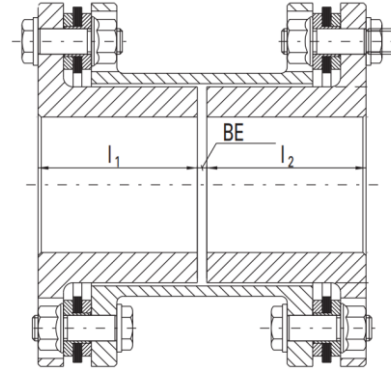
SSD-6 Types: Standard Configuration with Variable BE
