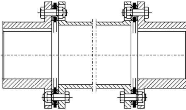
SSD-6 Types: Standard Configuration with Variable BE
