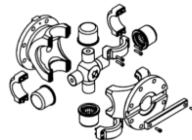
Figure 4 Split Eye
