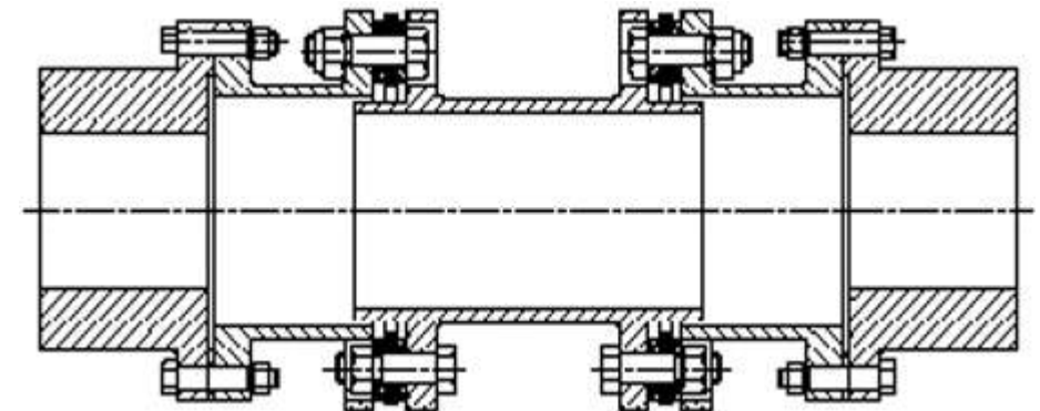
SSZ-6 Type: Drop-out Configuration with Floating Assembly
