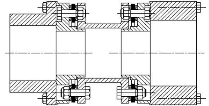
SAS-6 Type: Drop-Out Configuration According to API* 610
