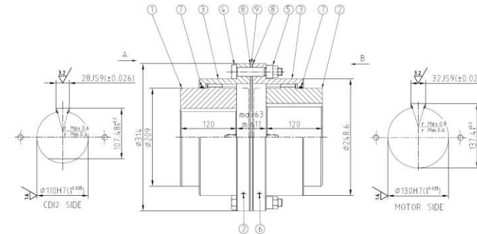
FGCO series coupling used for CDI Series equipment
