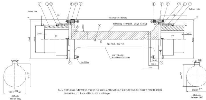
FGX-60-YY gear coupling used for ANDRITZ SCP HC refiner
