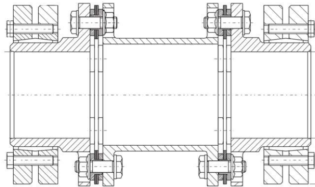
SSS-6 Type: Shrink Disc Configuration with Variable Distance between Shaft Ends
