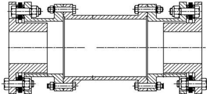
SRM-6 Type: Reduced Moment Configuration with Spacer according to AGMA* 516
