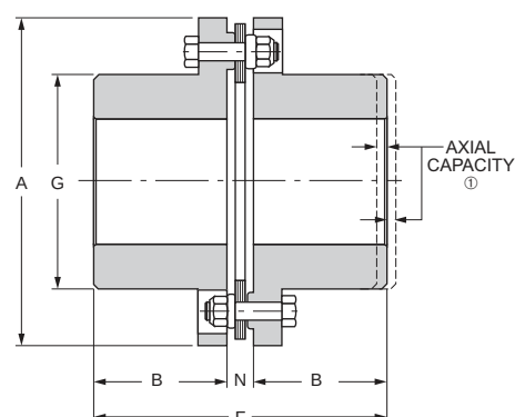
TYPE BMR SINGLE
