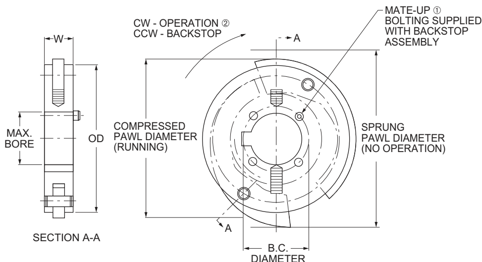
Bolt-On Backstop Tabulation (inch)
