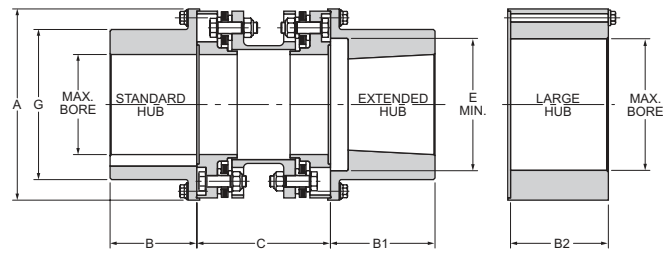
8 Bolt Design
