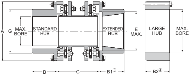
4 & 6 Bolt Design
