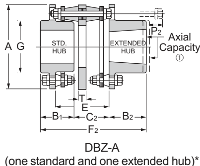
General Dimensions (inch)
