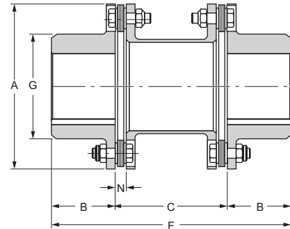
Series 52 TAPER BORES ALSO AVAILABLE
