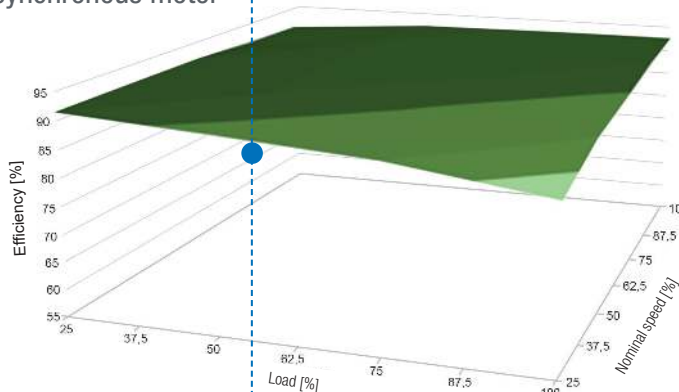
IE4 synchronous motor
