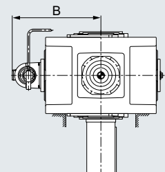
B4.V Forced lubrication by motor pump 2LP302-...22-....
