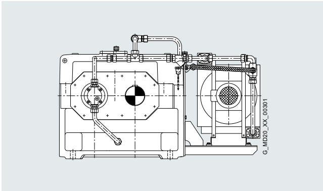
Example: H1SH07 with oil-air cooler, flange-mounted pump and pressure monitor
