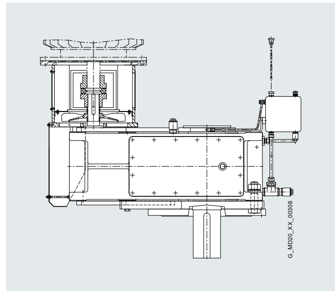
Example: H3SV11 – Lantern with integrated fan
