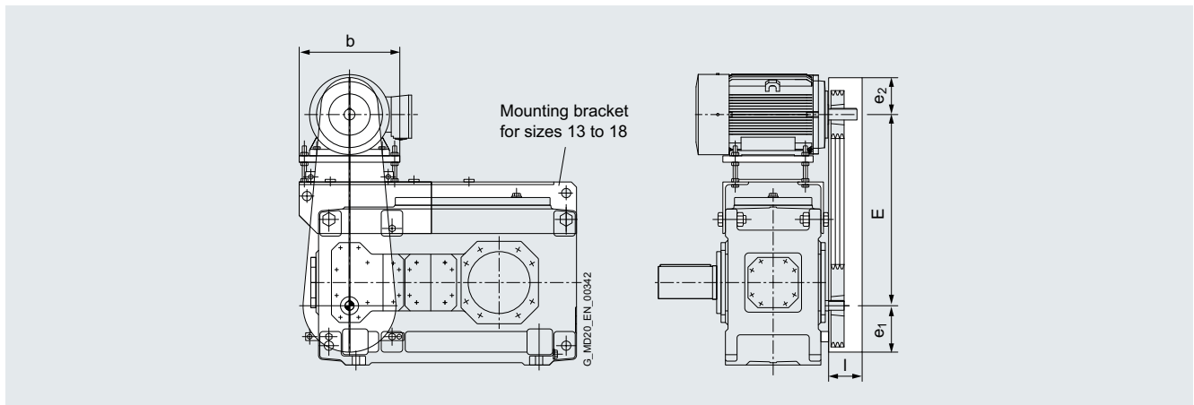
Piggy back for helical gear unit, horizontal installation, type H4
