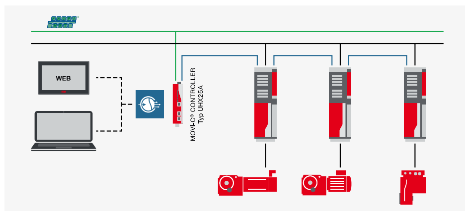
Device installation with MOVI-C® CONTROLLER, type UHX25A with MotionGateway
